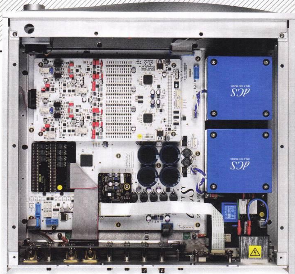
ABOVE: The 96 latches (a matrix of 2x48) that comprise the Ring DAC core are visible here with the two driving FPGAs sitting alongside [see boxout, p23]. The balanced analogue output lies to the left
