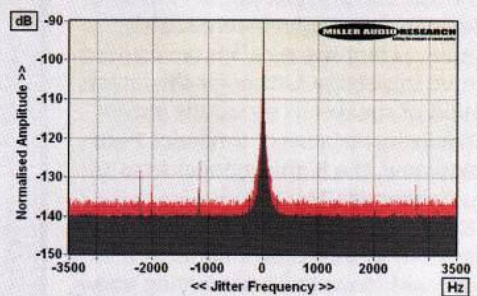
ABOVE: 24-bit/48kHz jitter spectra – 48kHz/24-bit over S/PDIF (black) and via network (red)
