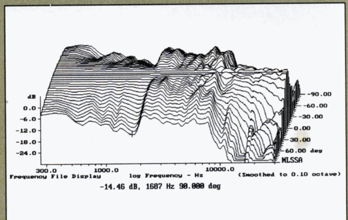
Fig.4 Vienna Acoustics Klimt The Kiss, lateral response family at 50°, normalized to response on tweeter axis, from back to front: differences in response 90–5° off axis, reference response, differences in response 5–90° off axis.
