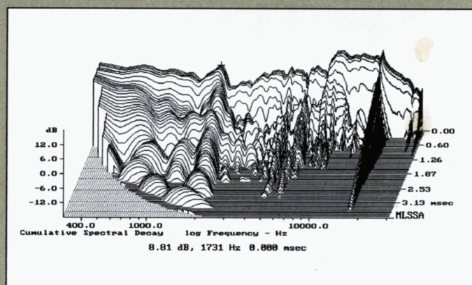
Fig.8 Vienna Acoustics Klimt The Kiss, cumulative spectral-decay plot on tweeter axis at 50" (0.15ms risetime).
