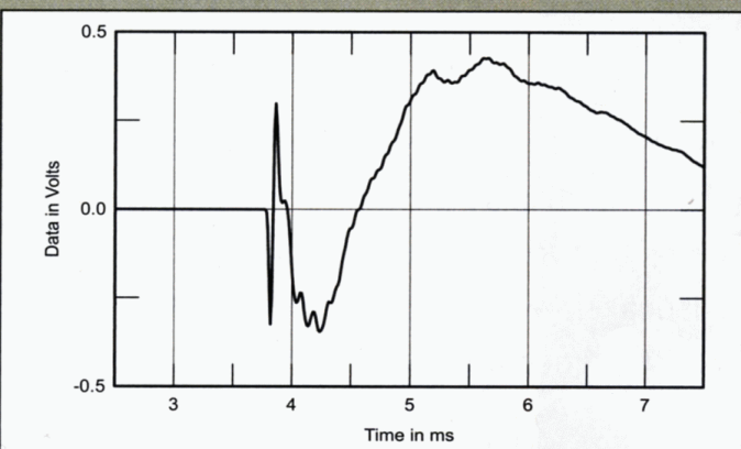
Fig.7 Vienna Acoustics Klimt The Kiss, step response on tweeter axis at 50" (5ms time window, 30kHz bandwidth).
