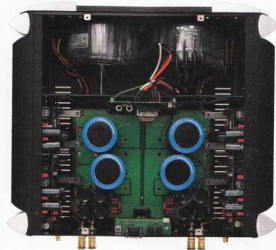
Dual-mono construction and two massive, custom-built transformers provide the grunt.
